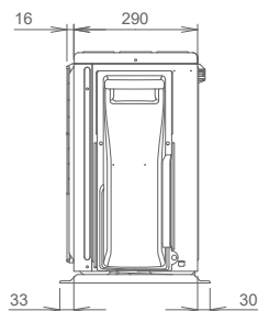
Air outlet
