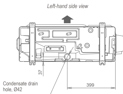
Underside view
