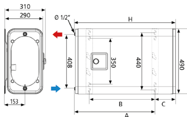
HORIZONTAL INSTALLATION
