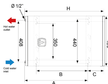
HORIZONTAL INSTALLATION
